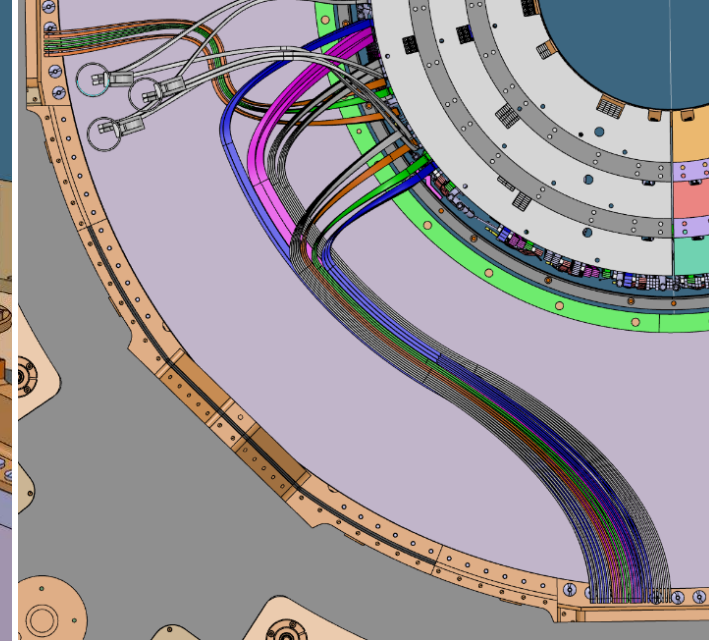
OUTER BARREL
