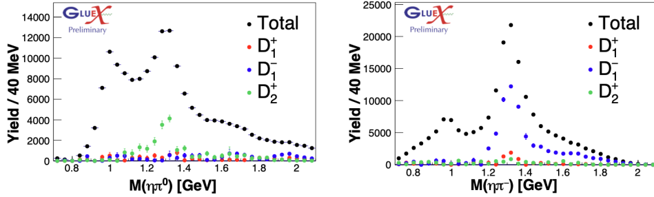
Fig. 2. – Preliminary results of a mass-independent partial wave analysis of the \eta\pi^0 (left) and \eta\pi^- final states in the momentum transfer range of 0.1 < |t| < 0.3 \text{ GeV}^2 . Only the dominant D -wave contributions are shown to illustrate the composition especially of the a_2(1320) signal.
