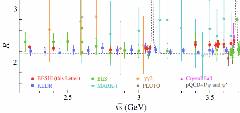
Fig. 2. – R values in the c.m. energy region from 2.2 to 3.7 GeV are reported. The red dots are the recent BESIII measurements and the other colours and symbols denote the previous experiments as detailed in the legend.
