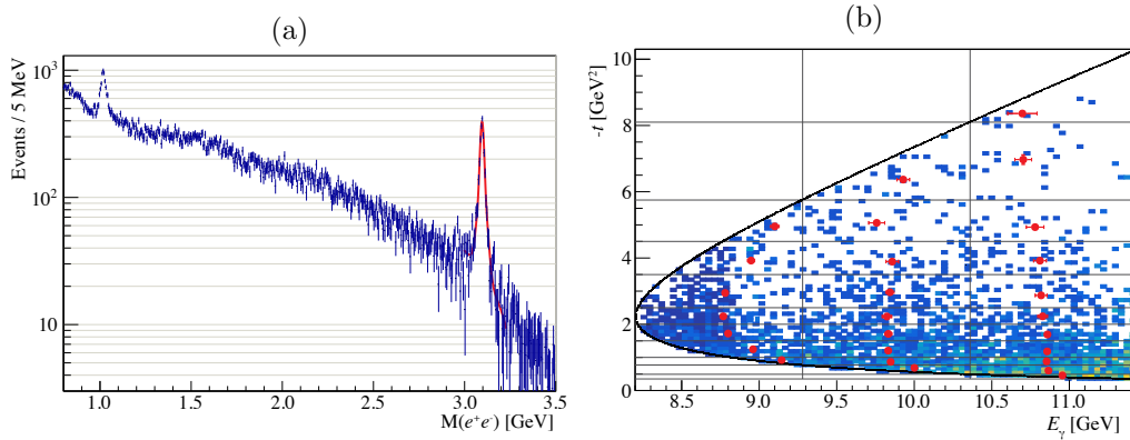
Fig. 2. – (a) - The mass spectrum of e^+e^- candidates (Ref. [2]). (b) - The flux-weighted E_\gamma - t distribution of the J/\psi candidates (Ref. [2]). For evaluation of the differential cross section the area was split into 3 bins in E_\gamma and 11 bins in t . The solid red dots show the average E_\gamma, t values per bin.
