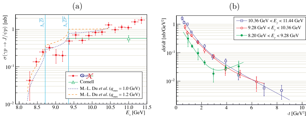
Fig. 3. – (a) - The measured full J/\psi cross section (Ref. [2]), compared with the calculations of open charm exchange [14]. The vertical lines indicate the energy thresholds for \Lambda_c \bar{D} and \Lambda_c \bar{D}^* production. (b) - The measured J/\psi differential cross section (Ref. [2]) in three beam energy intervals. The data are fitted with a sum of two exponential functions. At the lowest energy the second exponential contribution is significant.
