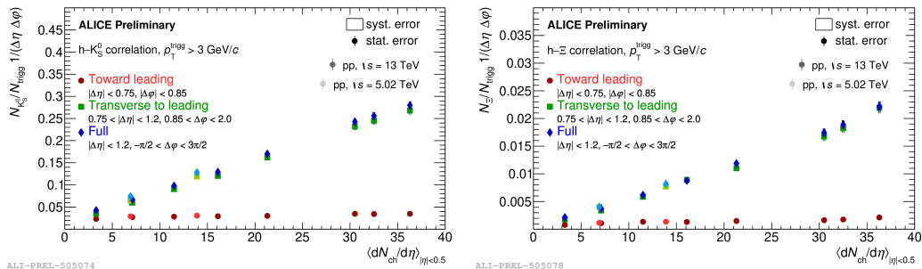
Fig. 4. – Ratio of K_s^0 (left) and \Xi^\pm (right) yields to unidentified-charged-trigger-particle yields as a function of charged-particle multiplicity density. The results for in-jet particles (red points) are compared with those of inclusive (blue points) and out-of-jet (green points) particles. Statistical uncertainties are represented by vertical error bars and systematic uncertainties by boxes.
