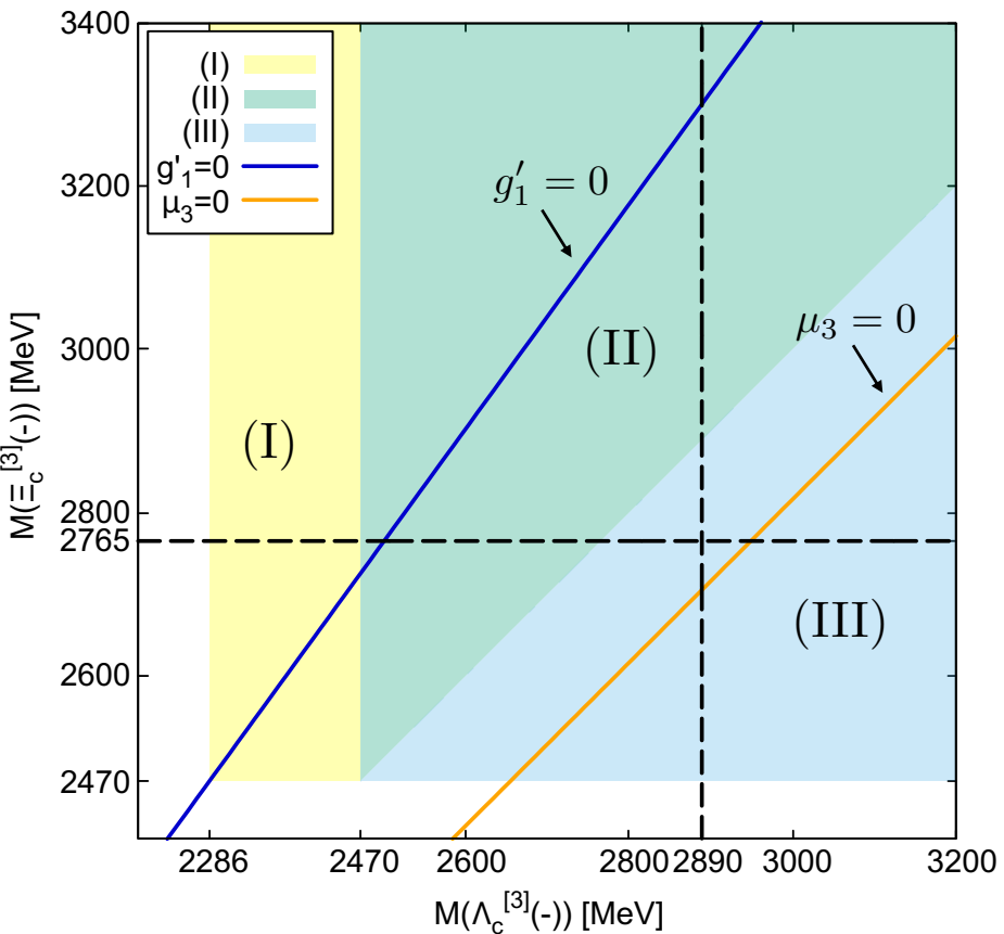
(a) The three mass hierarchies in Eq. (9).
