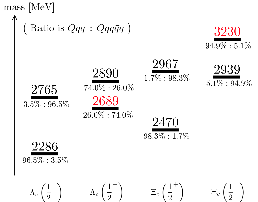
(b) The mass spectrum with the mixing effects.
