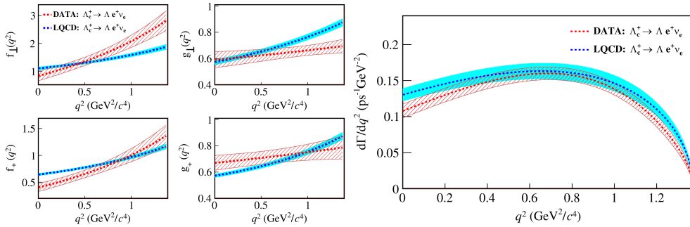
Fig. 1. – The left four figures show comparison of form factors with LQCD calculations. The bands show the total uncertainties. The right figure shows comparison of the differential decay rates with LQCD predictions. The band shows the total uncertainty.
