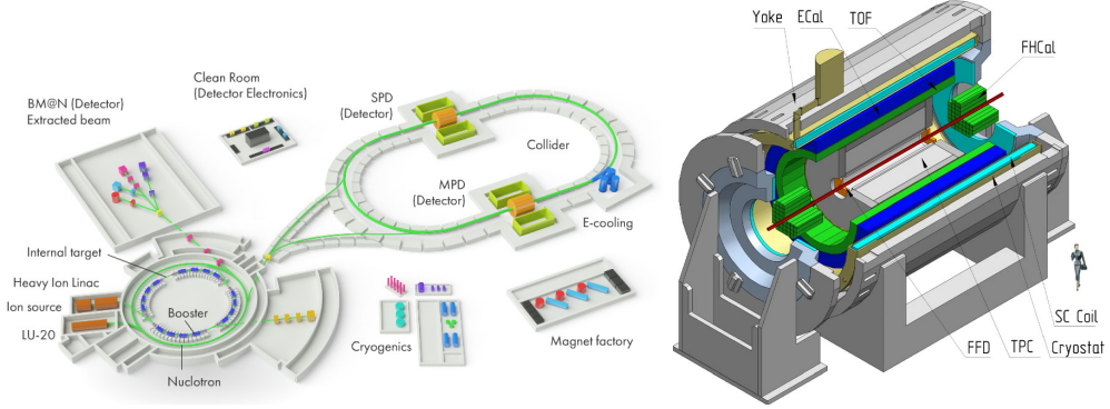
Fig. 1. – Schematic diagram of NICA complex (left), in which appears the main elements and first stage of MPD experiment (right).
