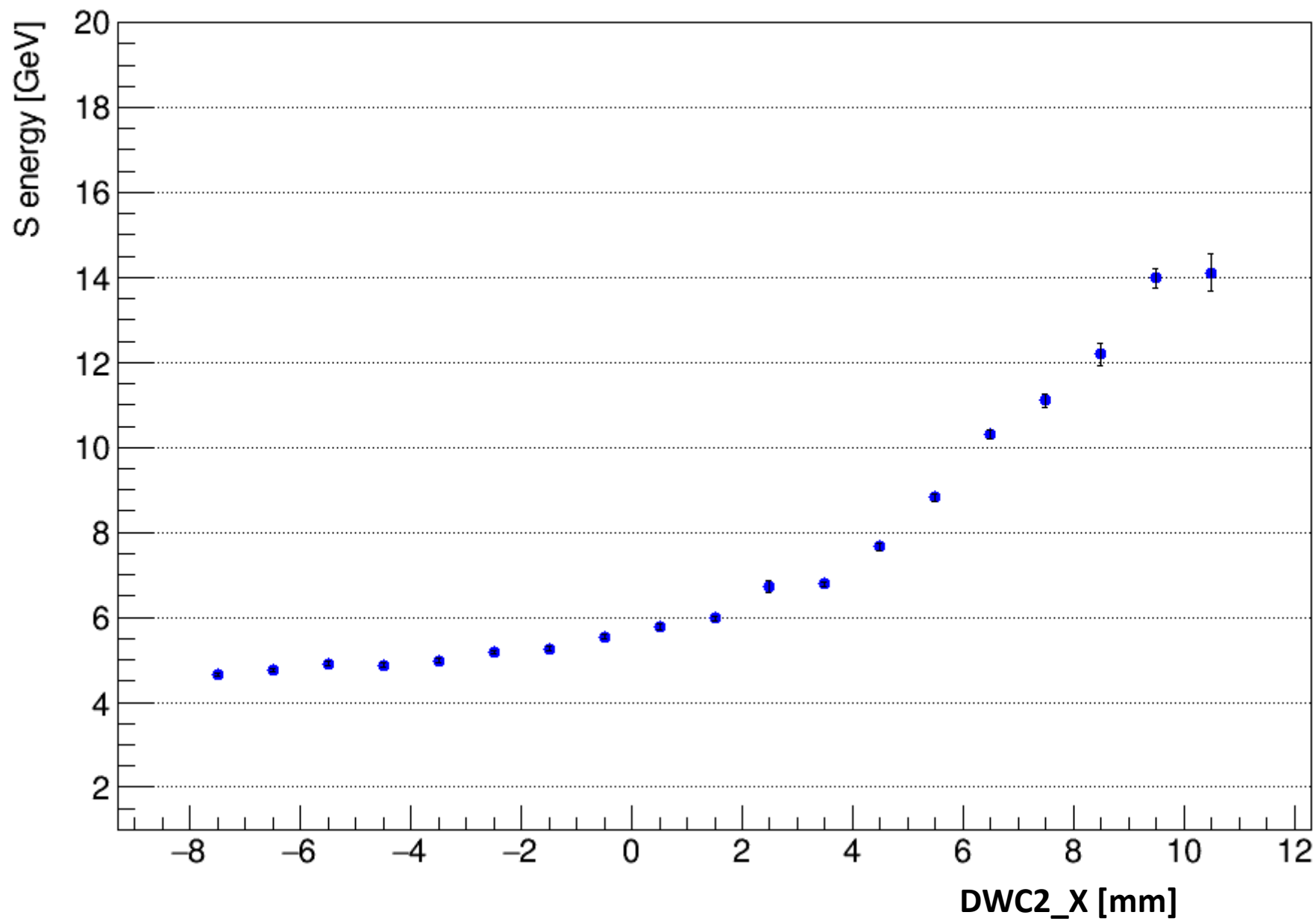
S energy in -10 \text{ mm} < Y < 10 \text{ mm} , 20 GeV run (PMTs)
