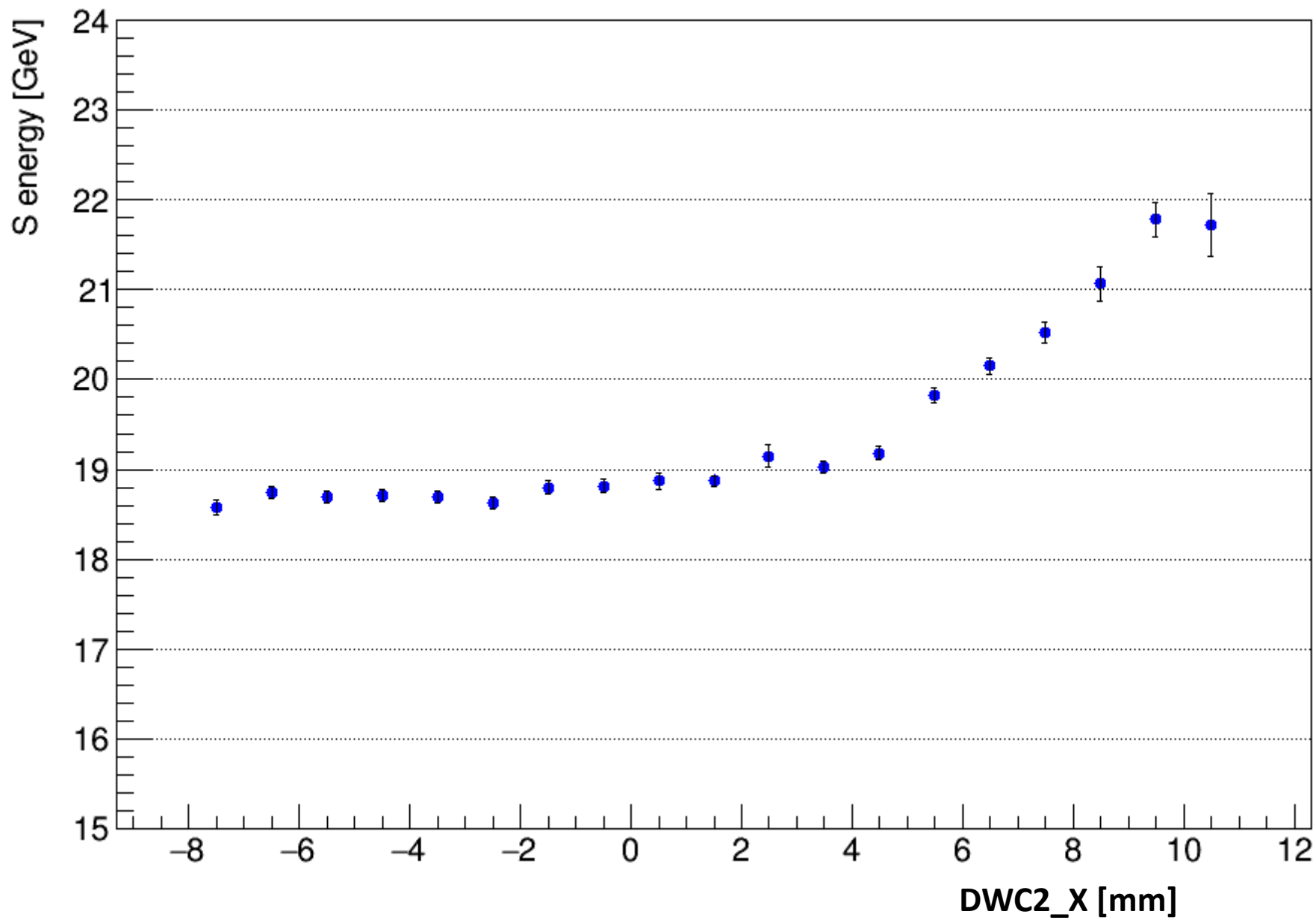
S energy in -10 \text{ mm} < Y < 10 \text{ mm} , 20 GeV run
