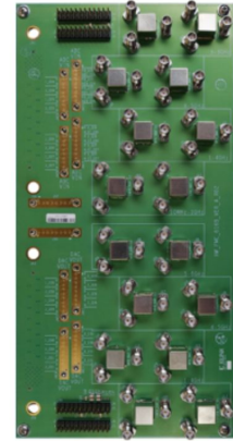
XM655 Breakout Add-on Card
