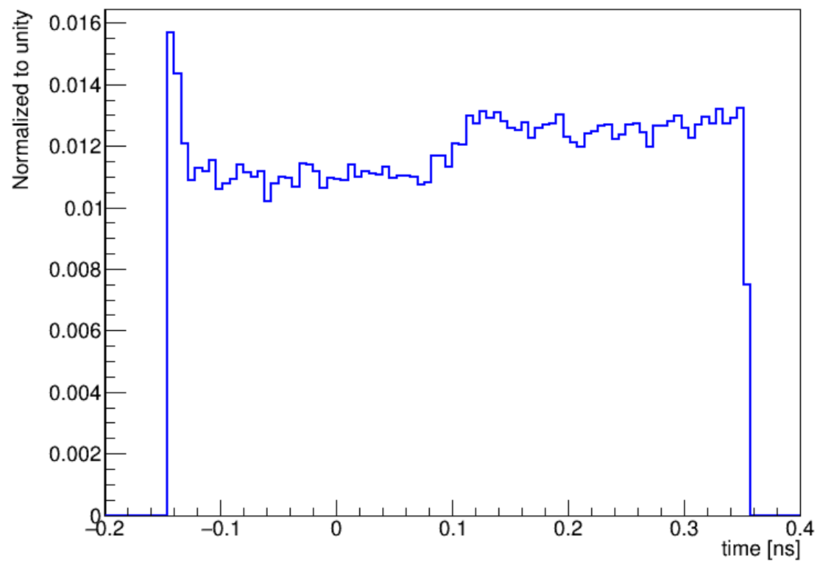
hit time in HCal Barrel
