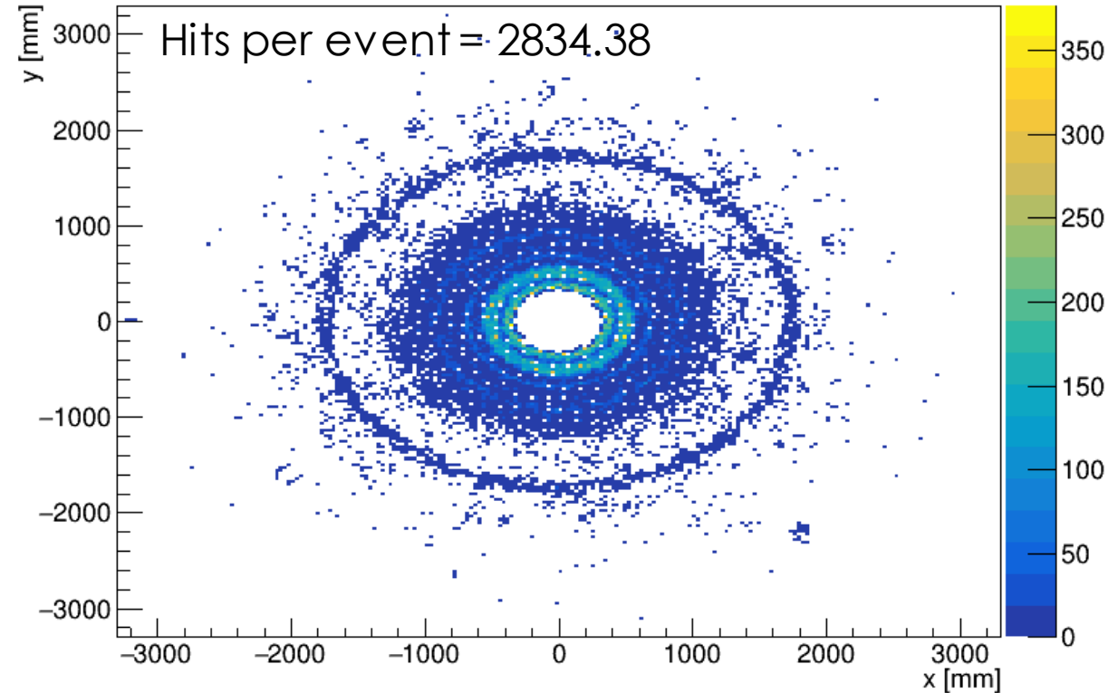
Hcal - Endcap Layers:10-15
