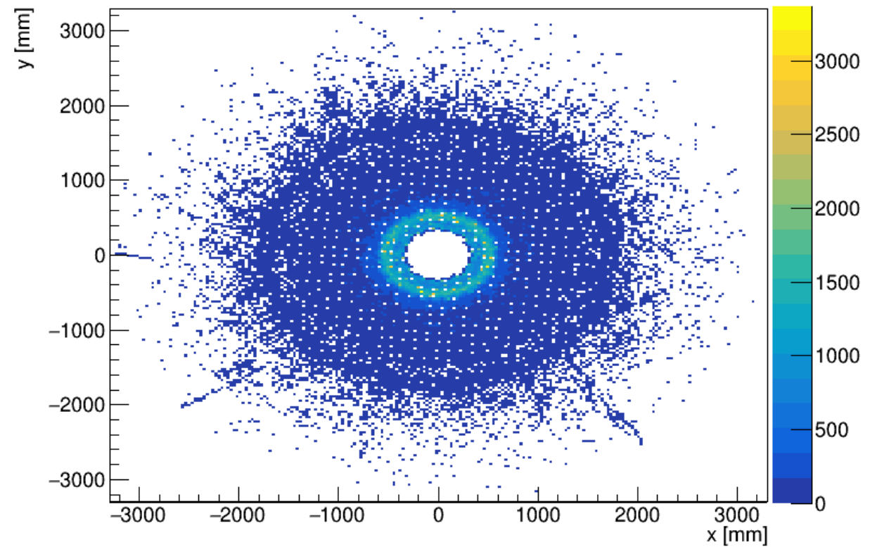
HCal - Endcap
