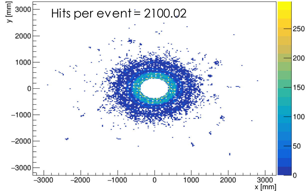
Hcal - Endcap Layers:30-35
