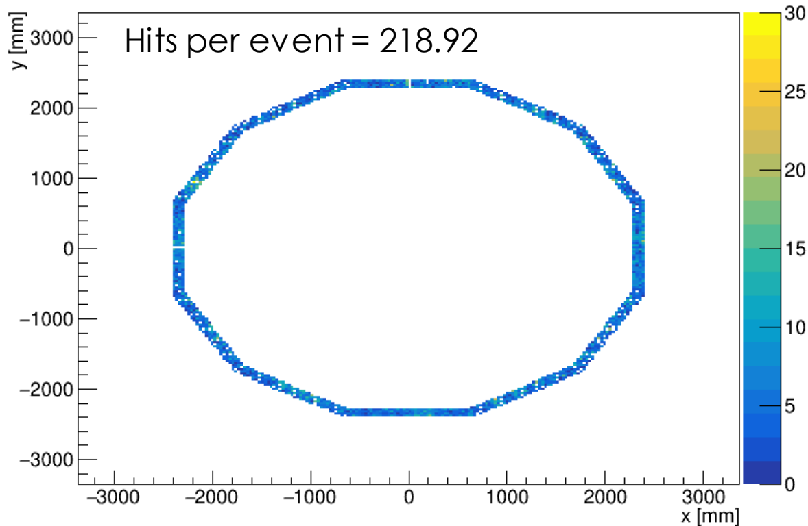
Hcal - Barrel Layers:20-25
