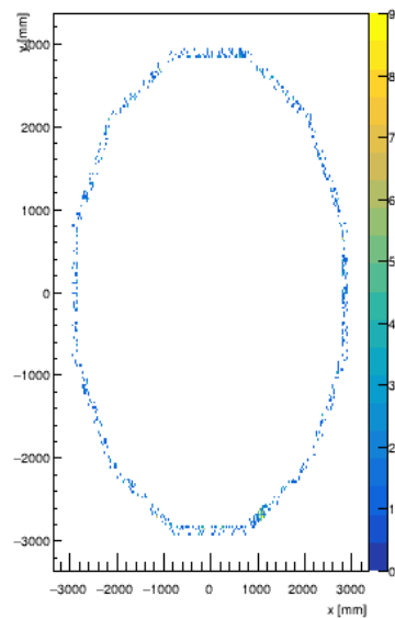
Hcal - Barrel Layers:40-45
