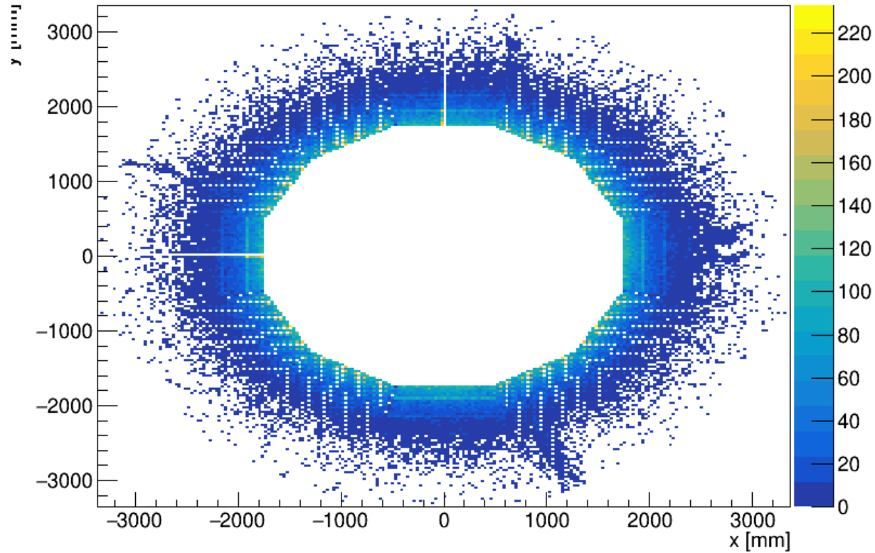
HCal - Barrel
