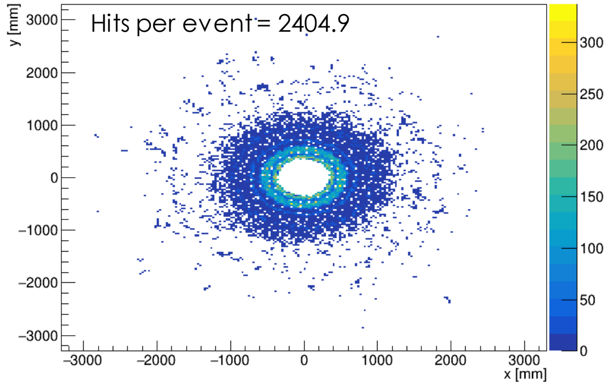
Hcal - Endcap Layers:20-25
