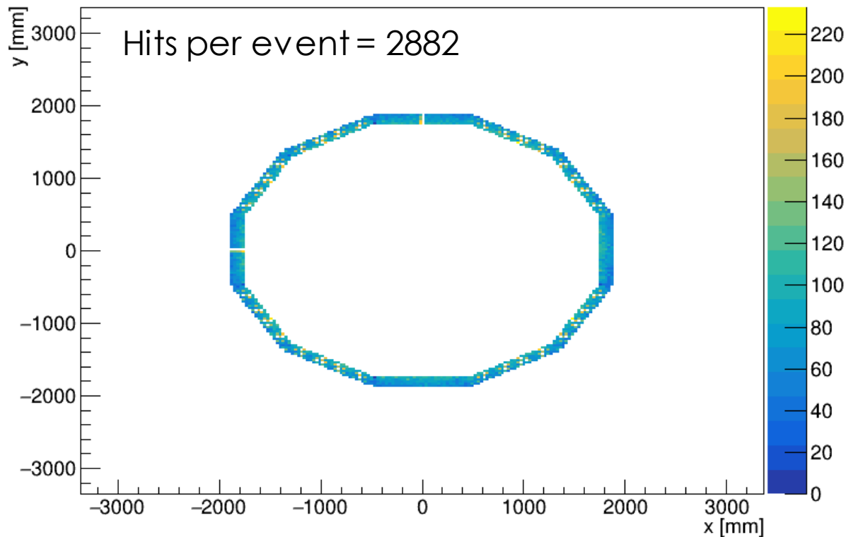
Hcal - Barrel Layers:0-5
