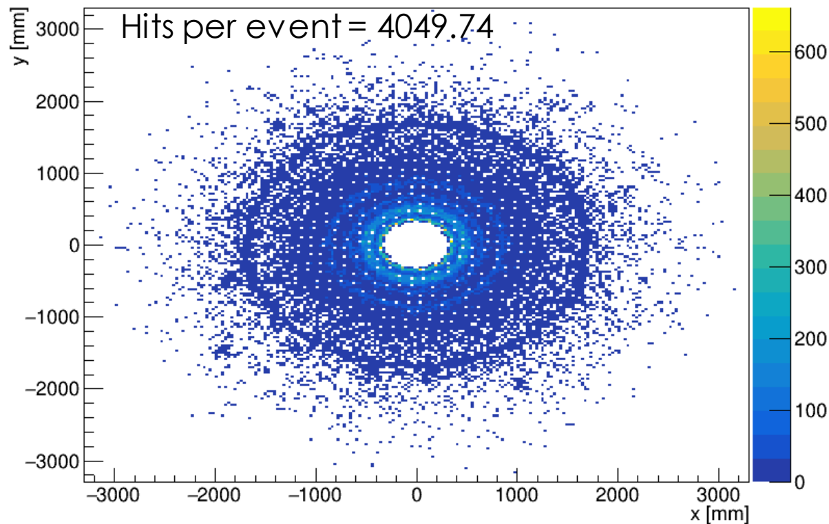
Hcal - Endcap Layers:0-5
