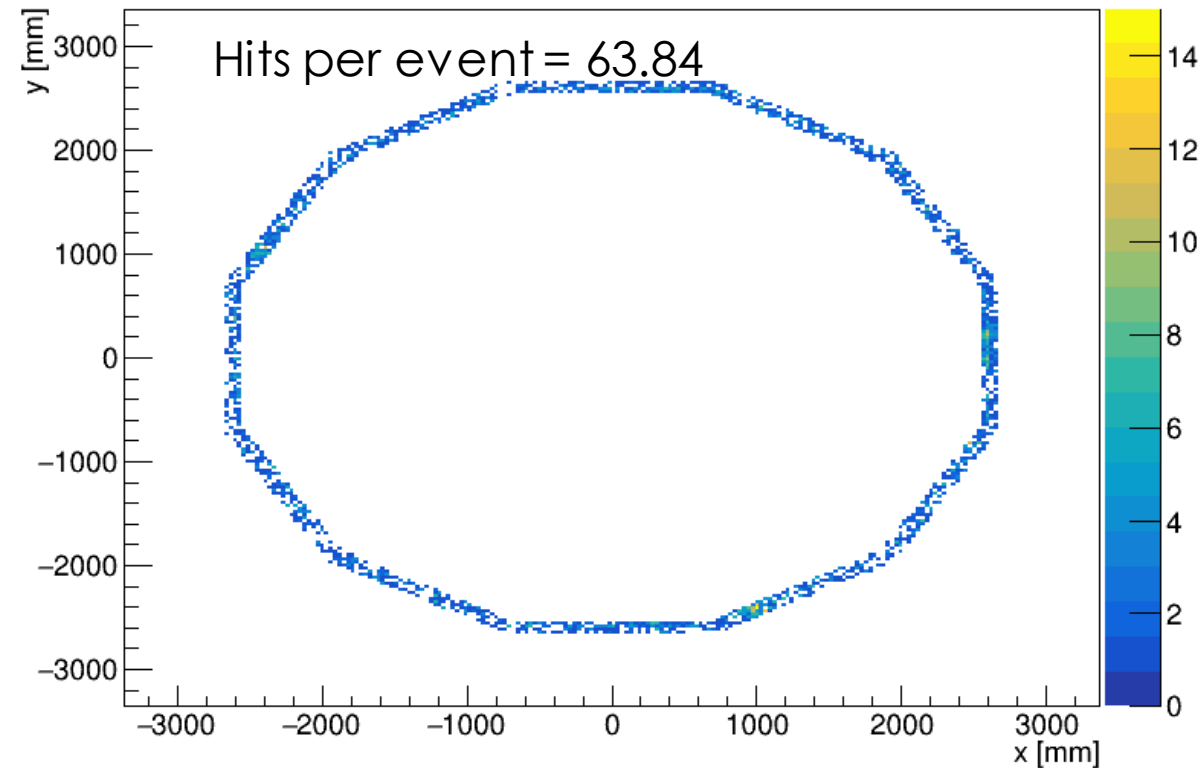
Hcal - Barrel Layers:30-35
