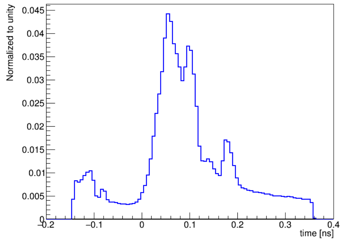
hit time in HCal Endcap
