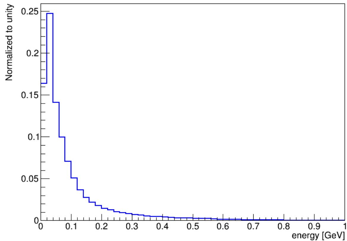
hit energy in HCal Barrel
