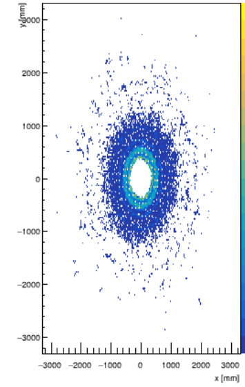
Hcal - Endcap Layers:20-25
