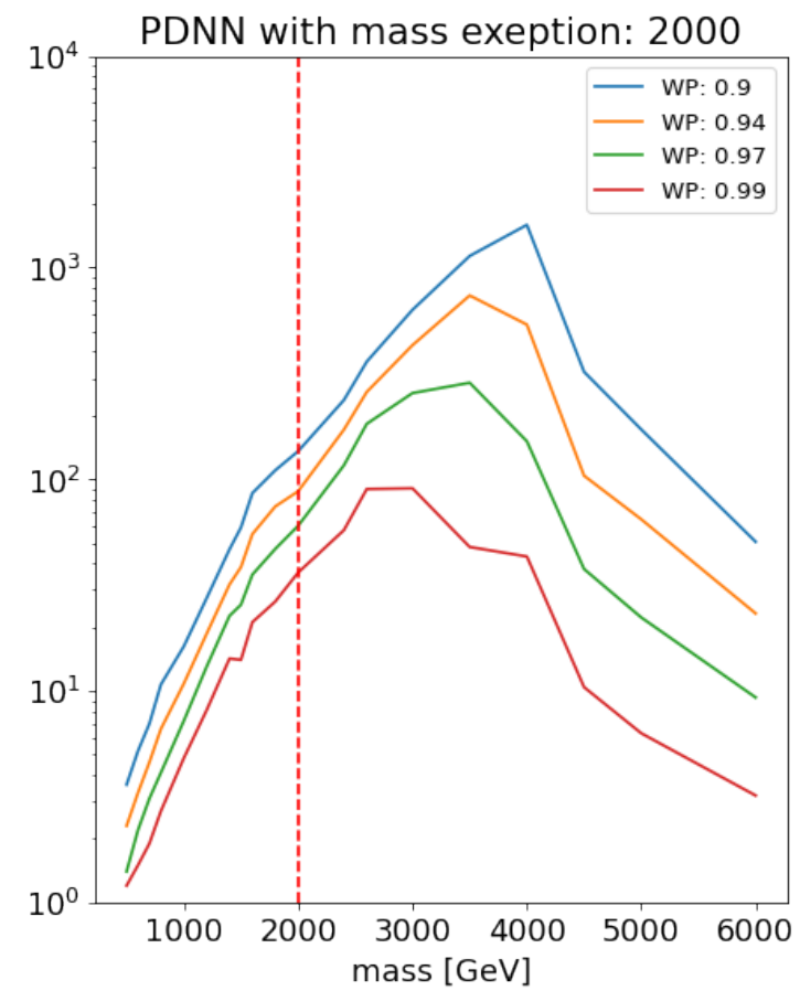
PDNN UFO_PFLOW_merged_ggF_Zjets_Diboson_Radion
