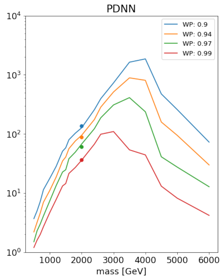
PDNN UFO_PFLOW_merged_ggF_Zjets_Diboson_Radion
