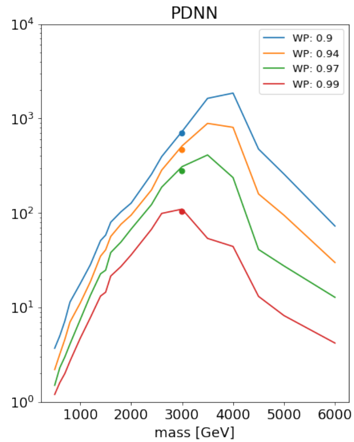
PDNN UFO_PFLOW_merged_ggF_Zjets_Diboson_Radion
