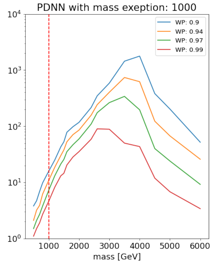
PDNN UFO_PFLOW_merged_ggF_Zjets_Diboson_Radion
