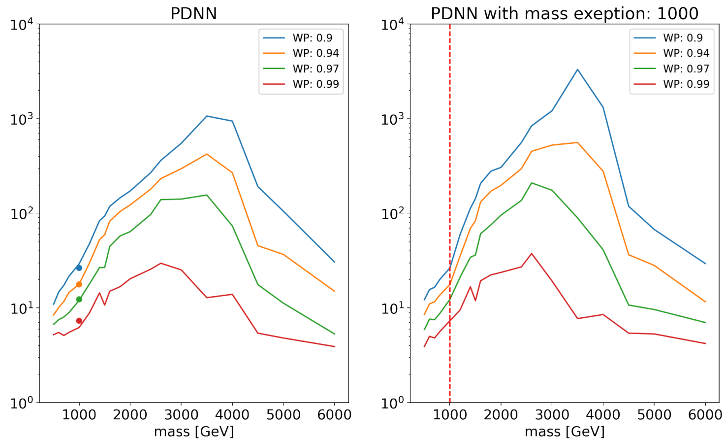
PDNN UFO_PFLOW_merged_ggF_Zjets_Diboson_Radion
