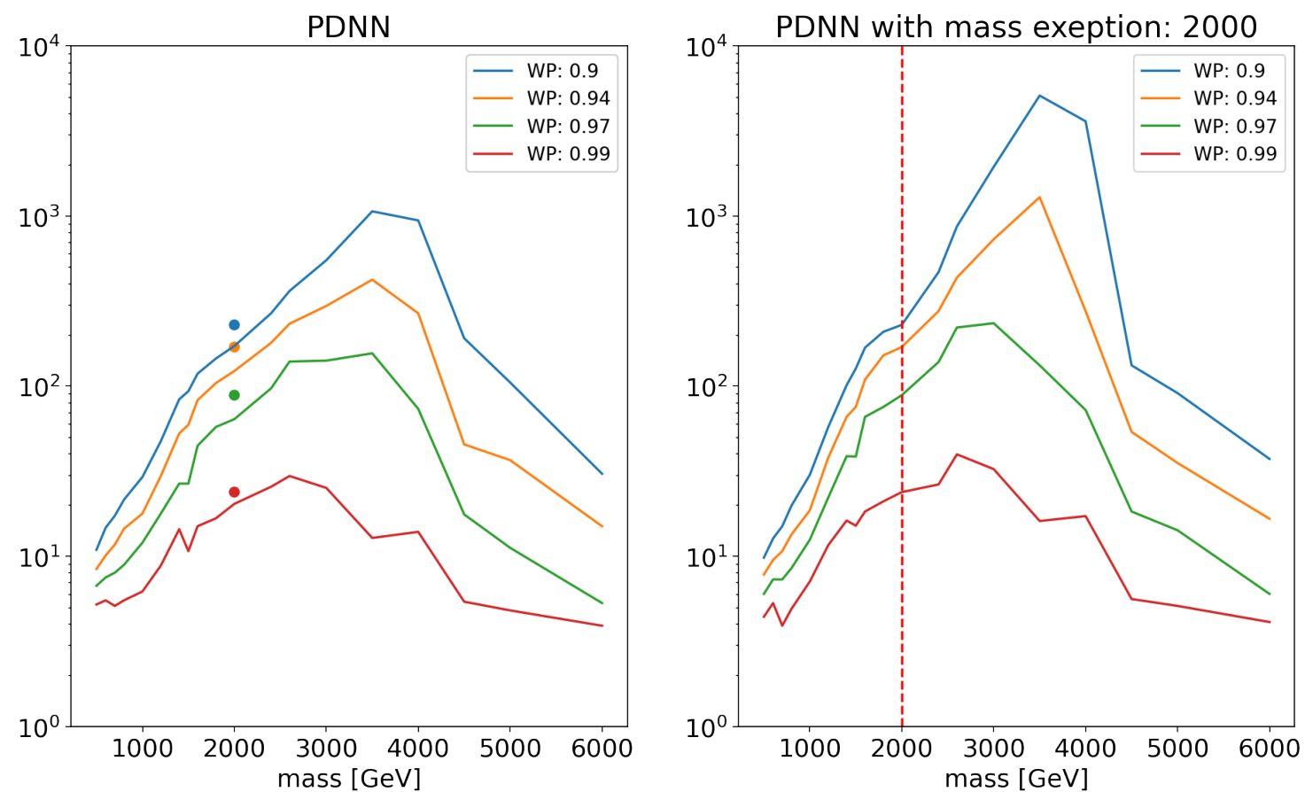
PDNN UFO_PFLOW_merged_ggF_Zjets_Diboson_Radion
