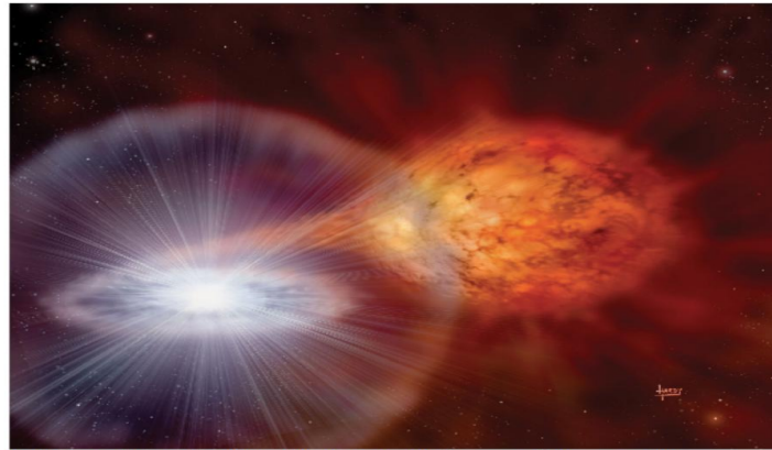
Artist's rendition of a white dwarf accumulating mass from a nearby companion star. This type of progenitor system would be considered singly-degenerate.
