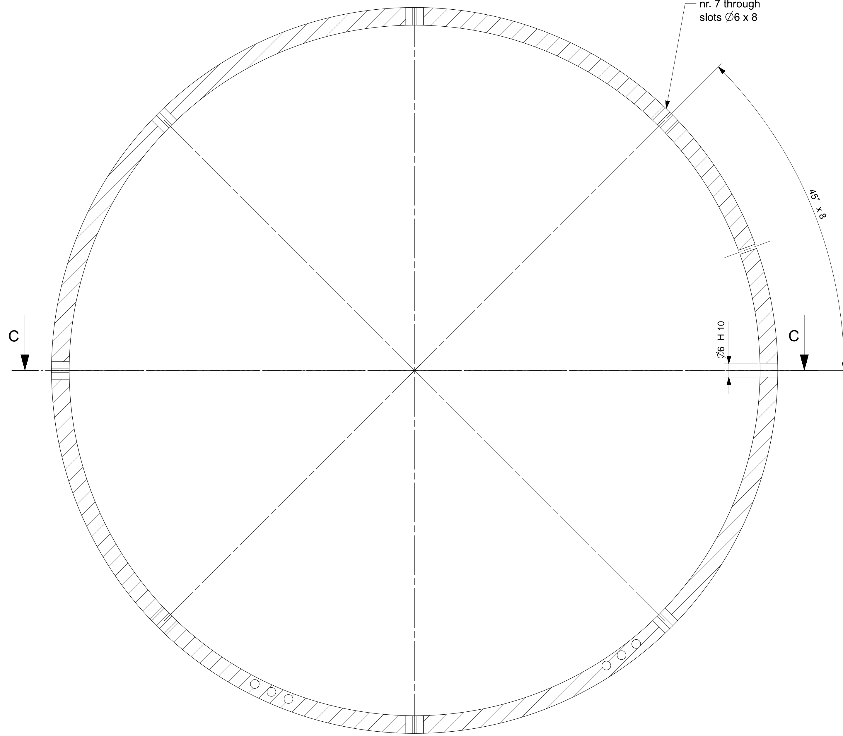
SECTION B-B
