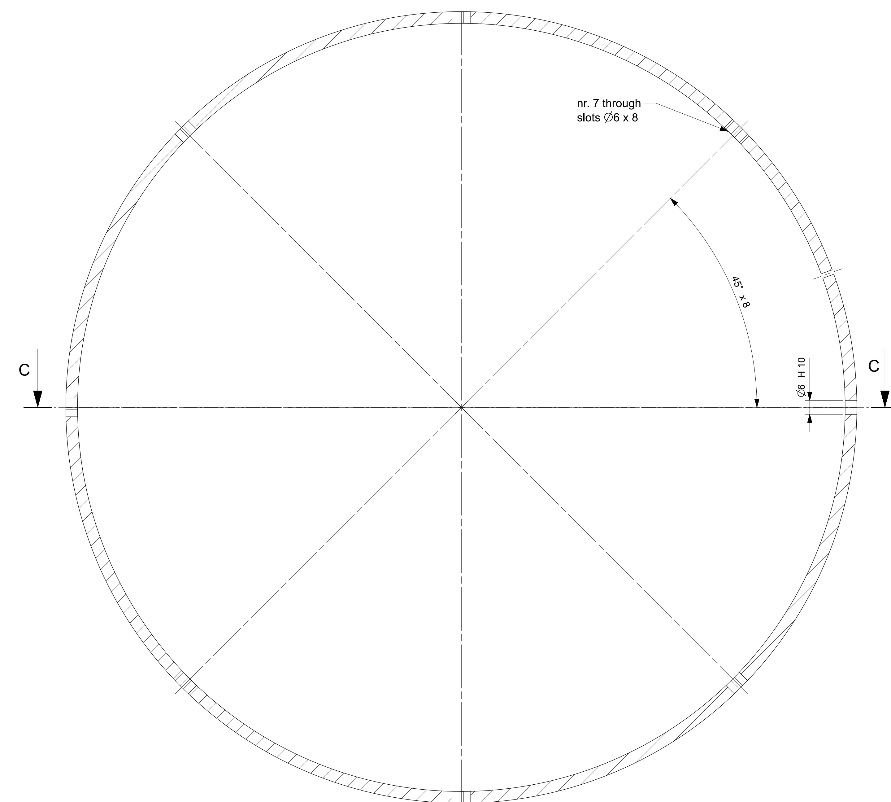
SECTION B-B
