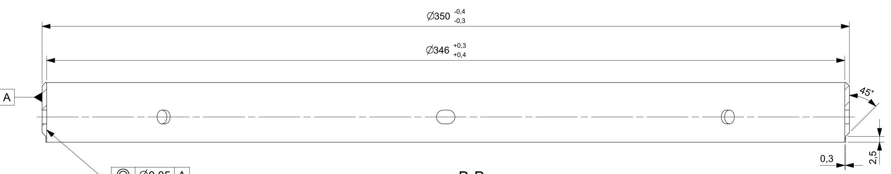
SECTION B-B
