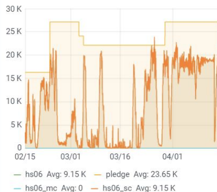
belle - HS06 & Pledge
