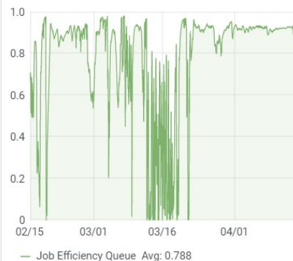
belle - Job Efficiency
