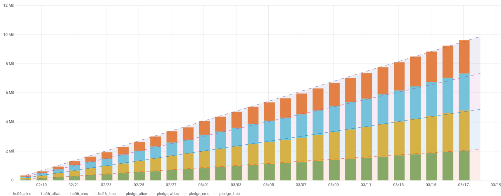
HS06_per_group cumulative
