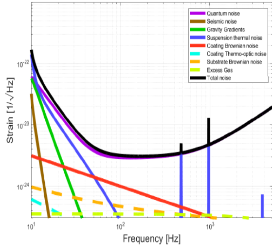
AdvLIGO Noise Curve: P_{in} = 125.0 W
