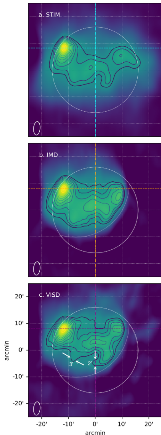
Fig. 5. Three LOFAR maps produced using three different methods. (a) A CLEAN map made via standard interferometric imaging (STIM) at 10:59 UT. (b) A map made by summing the Im_{diff} produced by differencing consecutive CLEAN maps, 1 minute apart (IMD). (c) A map made by summing the Im_{diff} , made by differencing consecutive visibility data, 1 minute apart (VSD). Each map is normalised and the contours are 50–95 % the max intensity. The solid white circle is the visible solar limb. The white crescent is the area not de-occulted by the moon.
