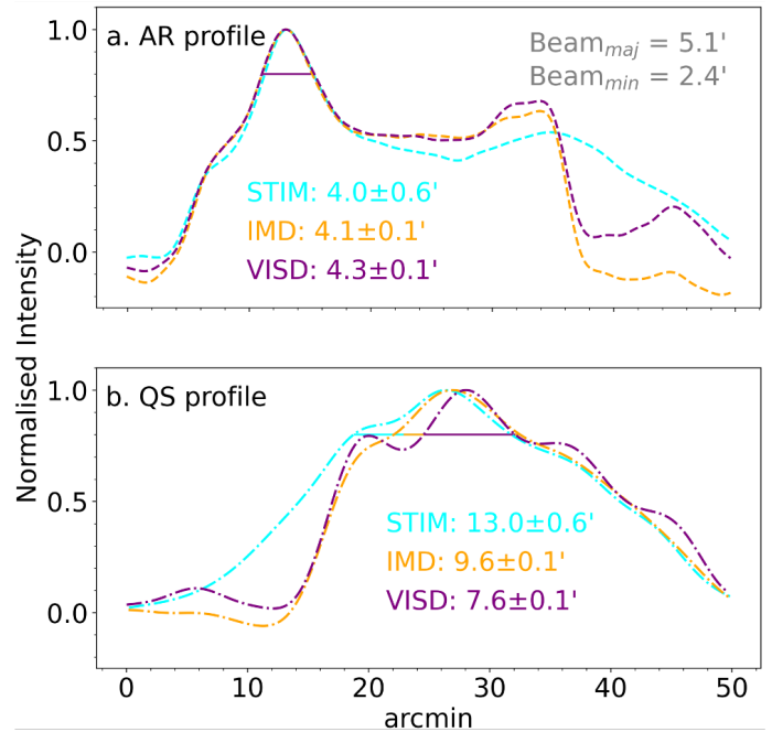
Fig. 6. Plot of the intensity slices across the bright active region (AR) emission corresponding to NOAA 12303 (---) and the quiet Sun (QS) emission (—). The profile colours correspond to the horizontal and vertical, coloured, dashed lines in Figure 5(a)–(c). The widths have been determined for the tallest peak, in each profile, as is labelled above.
