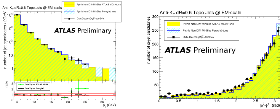
Fig. 1. – Jet distributions obtained at the electromagnetic scale; Left: Transverse momentum p_T at the electromagnetic scale; Right: Azimuthal angle difference \Delta\phi of the two most energetic jets in the event.
