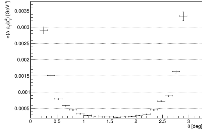
\mu sample with p=10 GeV
