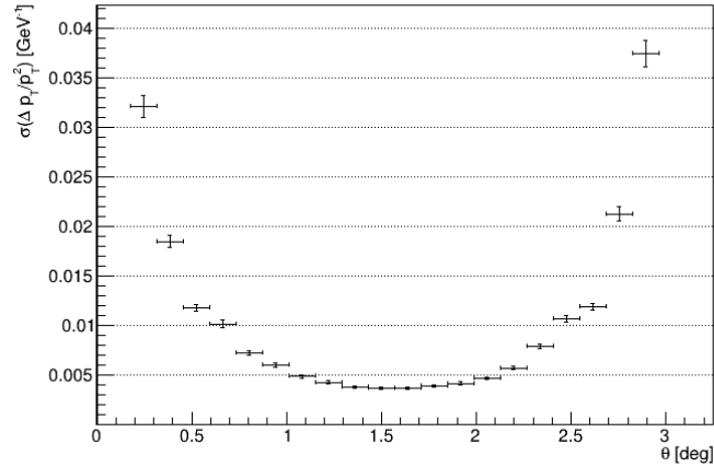
\mu sample with p=1 GeV
