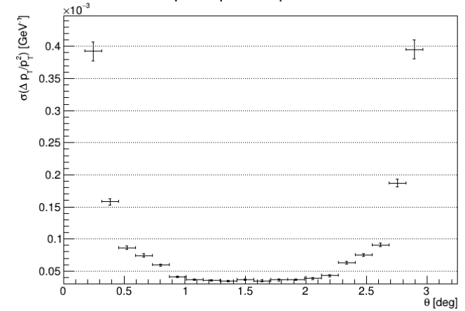
\mu sample with p=100 GeV
