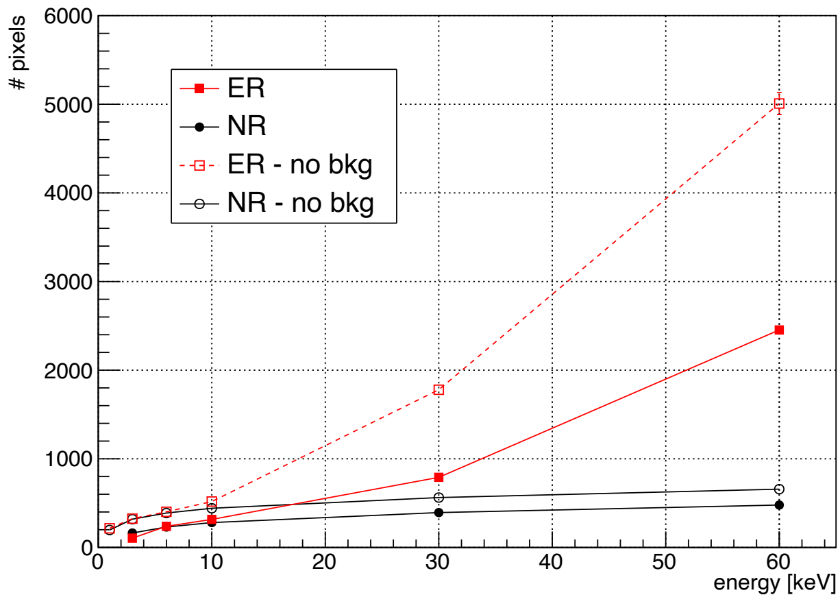
Clusters # pixels vs energy
