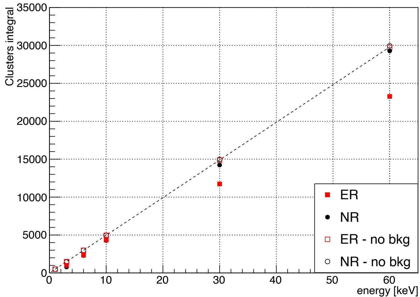
Clusters integral vs energy
