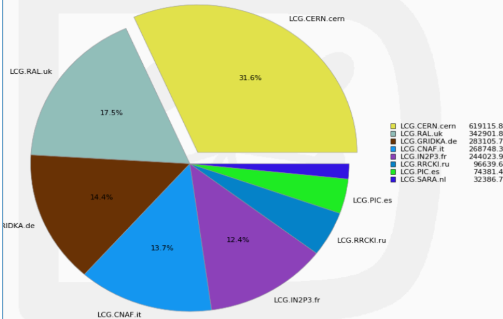
CPU days used by Site 8 Weeks from Week 20 of 2020 to Week 28 of 2020
