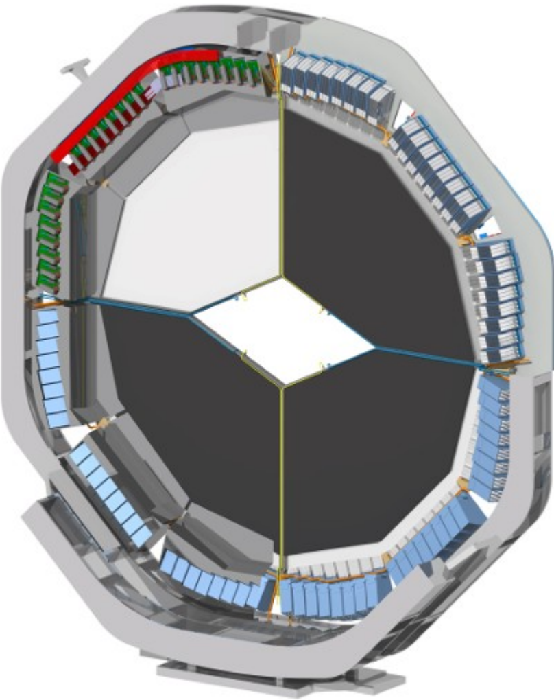
EDD cut-away view from downstream
