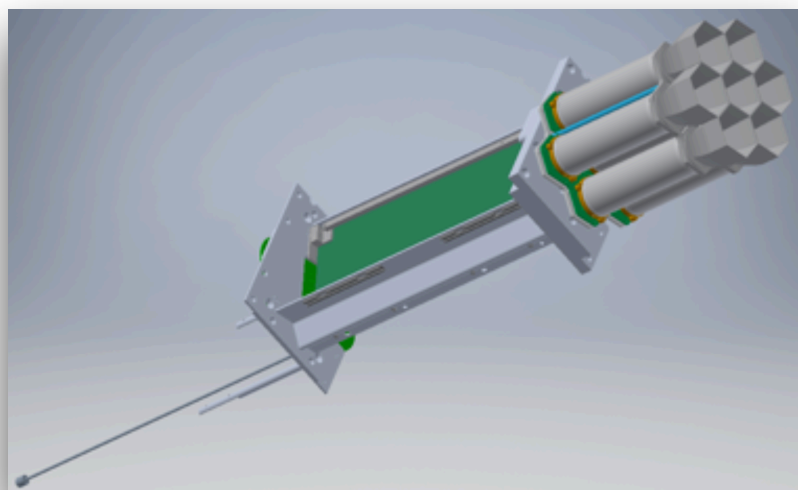
Mechanical structure of a PMT cluster for LST
