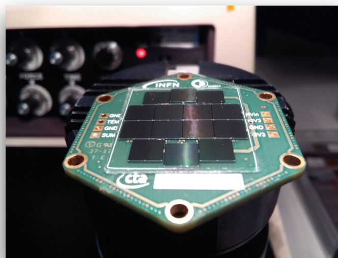
Design e characterization of a pixel: 14 SiPMs FBK NUV HD3_2
