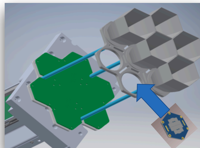
Mechanical structure for a SiPM cluster
