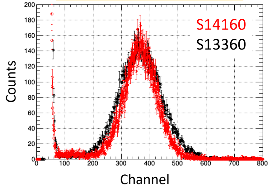
BGO (241Am 60 keV)
