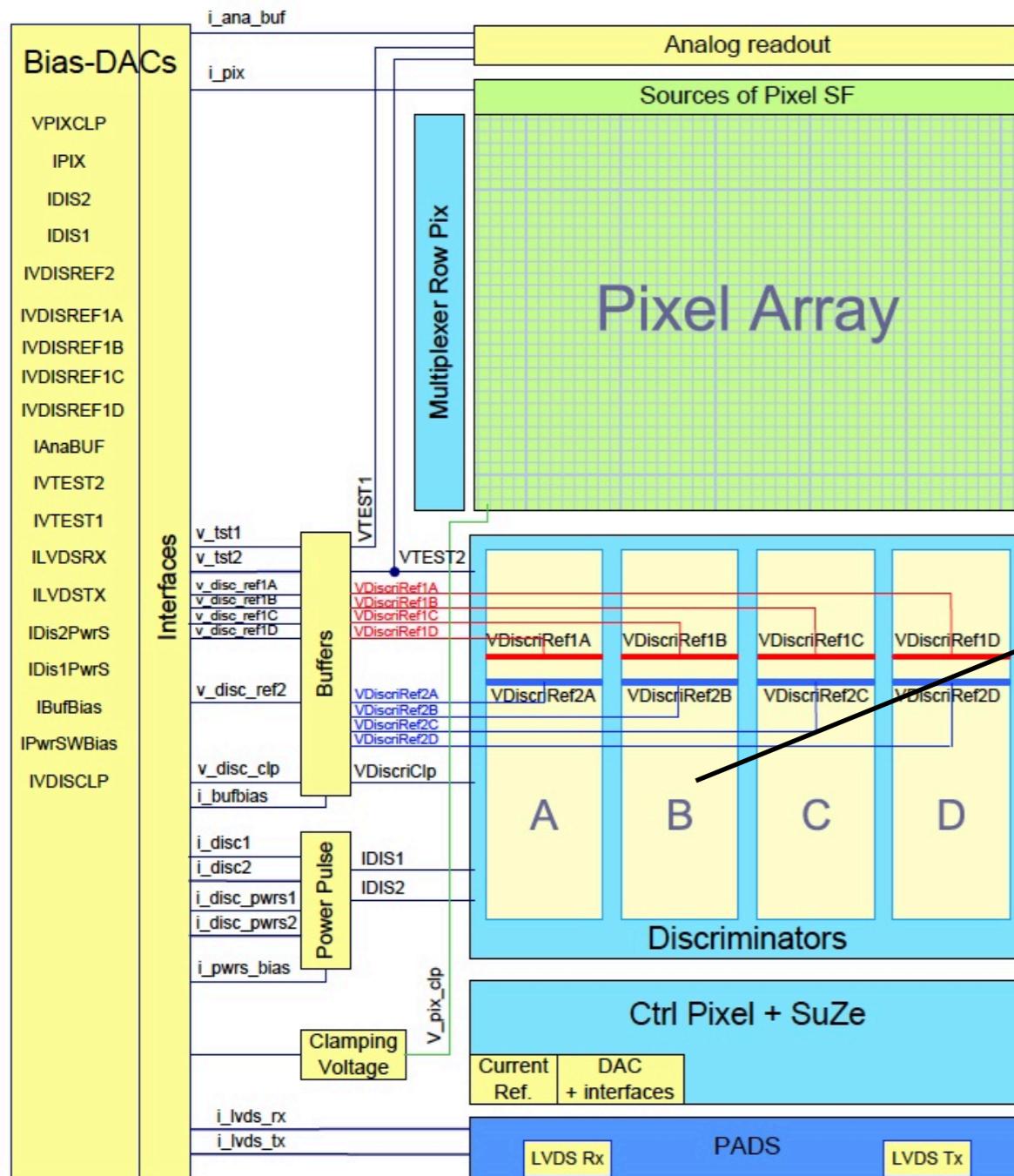
Figure 19: Bias synthetic bank diagram
