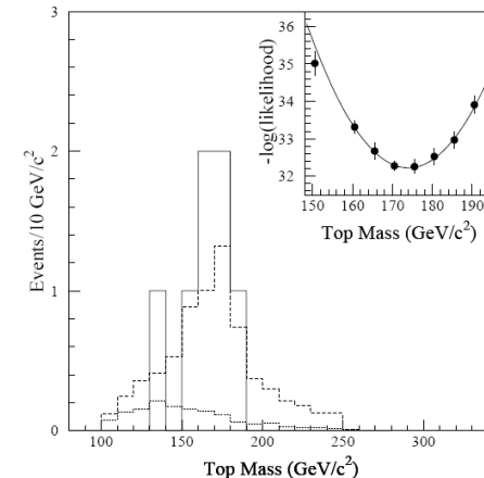
Top: high p_T leptons and jets, MET, b tagging
