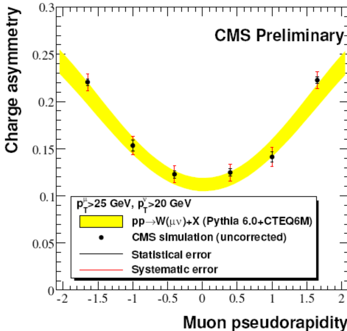
Figure 5: The measured charge asymmetry for 100 \text{ pb}^{-1} of simulated luminosity. The systematic error is dominated by the statistical error on the efficiency ratio determined using 100 \text{ pb}^{-1} of Drell-Yan MC. 51
