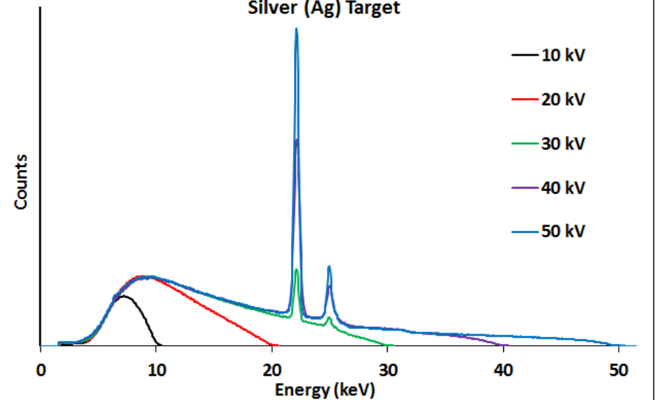
Mini-X Output Spectrum at Different Voltages: Silver (Ag) Target
