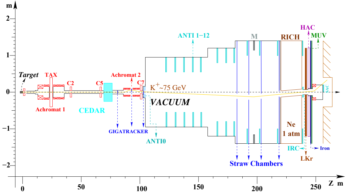
Figure 4: Layout of NA62 experimental apparatus.
