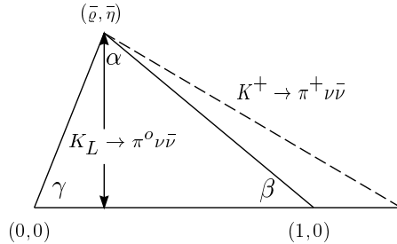
Figure 2: Connection between the branching ratios of K \rightarrow \pi\nu\bar{\nu} decays and the unitarity triangle.
