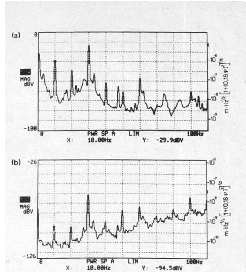
FIG. 6. The, RA locked-, open- (a), and closed- (b) loop frequency spectra for 0 < \nu < 100 Hz.
