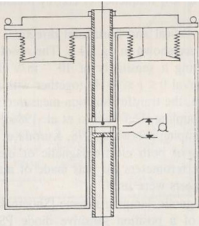
Fig. 11.5. The schematic diagram of a gas spring (from Del Fabbro et al. [1988a]). The gas pressure pushes the bellow piston, a load attached to the lower wire. A rigidity of 34 \times 10^3 N/m with four bellows and of 20 \times 10^3 N/m with two bellows was obtained.
