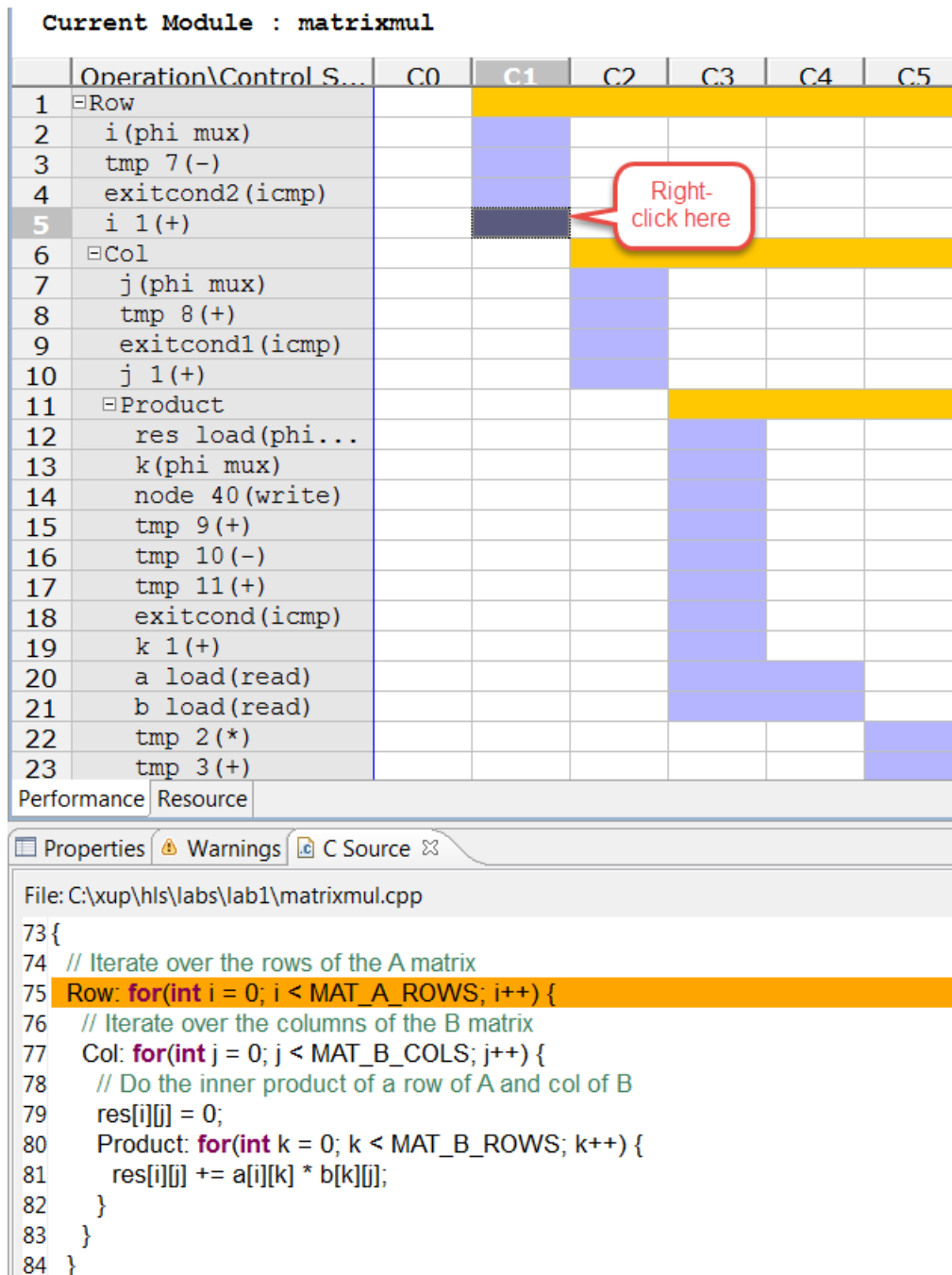
Figure 17. Cross probing into the source file
