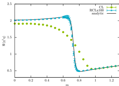
\langle \eta^\dagger \eta \rangle for \mu = 1 and n = 24
