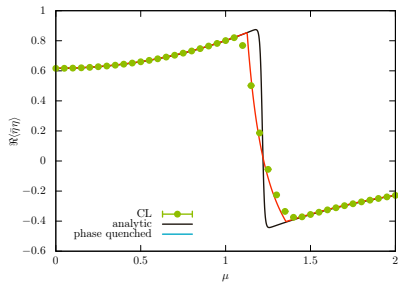
\langle\bar{\eta}\eta\rangle for m = 1
