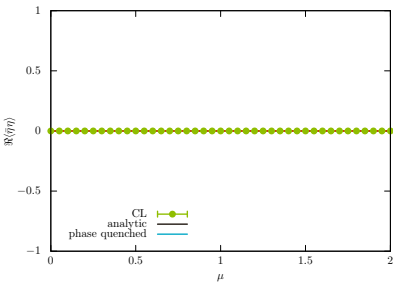
\langle\bar{\eta}\eta\rangle for m = 0
