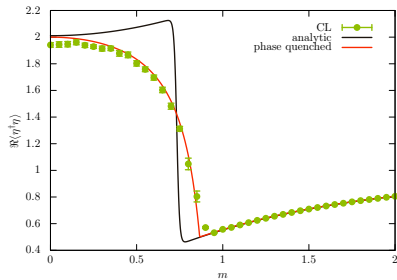
\langle\eta^\dagger\eta\rangle for \mu = 1
