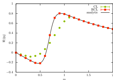
\langle \bar{\eta} \eta \rangle for \mu = 1 and n = 6
