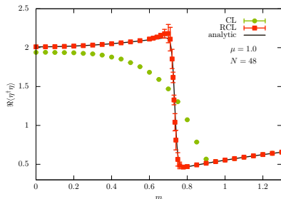
\langle \eta^\dagger \eta \rangle for \mu = 1 and n = 48
