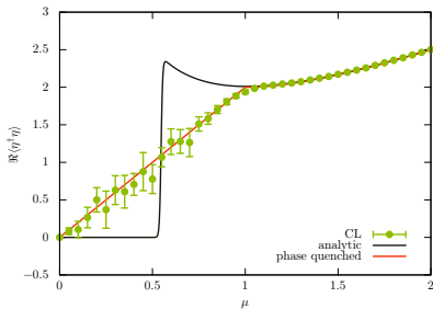
\langle\eta^\dagger\eta\rangle for m = 0
