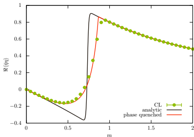
\langle\bar{\eta}\eta\rangle for \mu = 1
