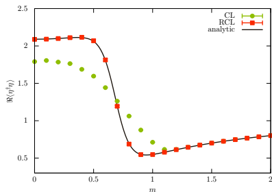
\langle \eta^\dagger \eta \rangle for \mu = 1 and n = 6
