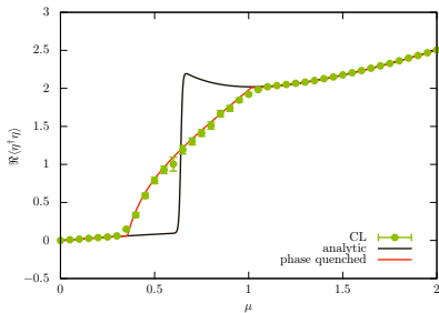
\langle\eta^\dagger\eta\rangle for m = 0.2
