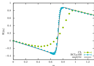
\langle \bar{\eta} \eta \rangle for \mu = 1 and n = 24
