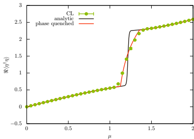
\langle\eta^\dagger\eta\rangle for m = 1
