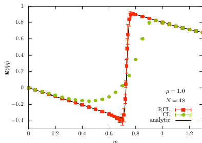
\langle \bar{\eta} \eta \rangle for \mu = 1 and n = 48
