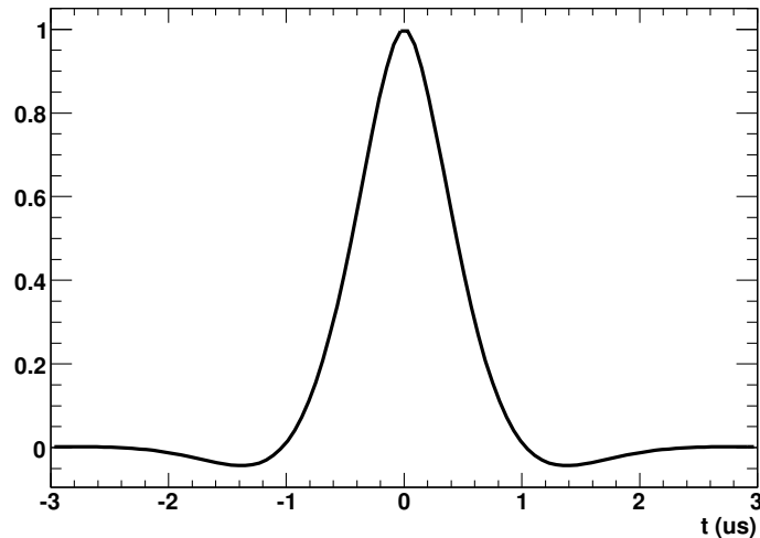
Shaped pulse with CsI(Tl) filter
