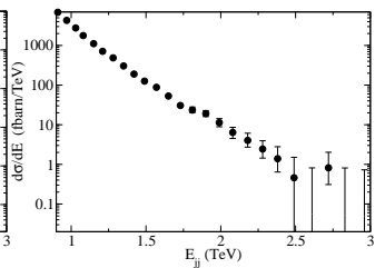
CMS WW events
