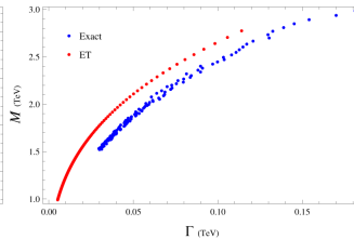
(b) Vector
