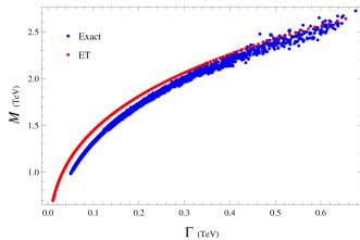
(a) Scalar
