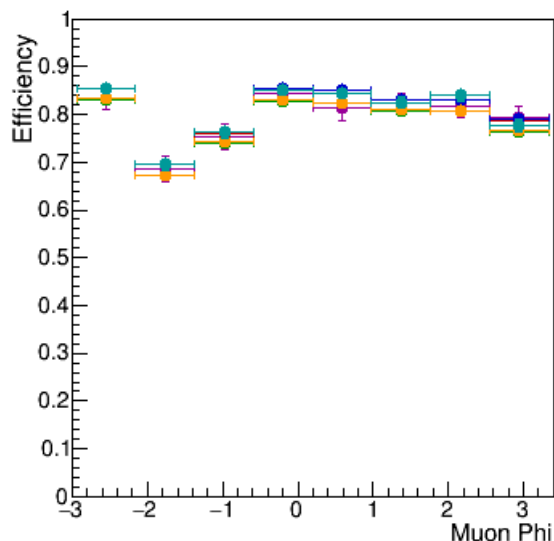
BARREL, Phi dependence
