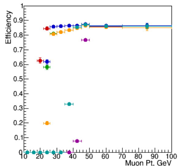
ENDCAP, Pt dependence
