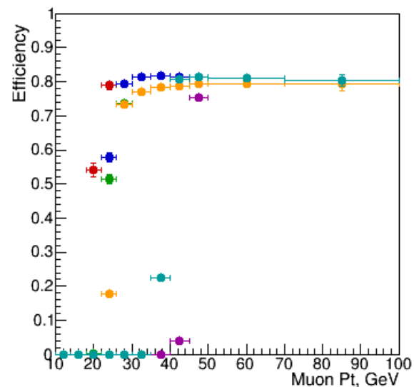
BARREL, Pt dependence
