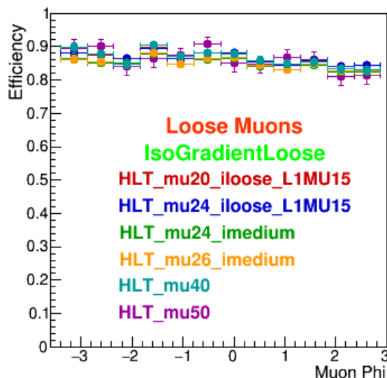
ENDCAP, Phi dependence
