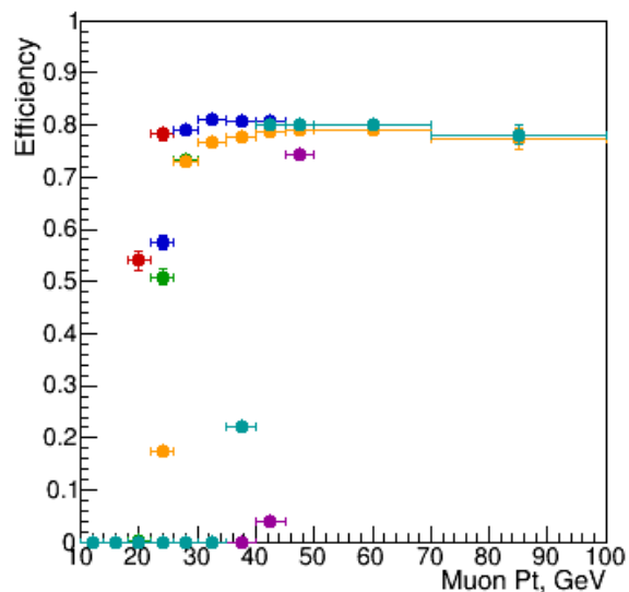
BARREL, Pt dependence
