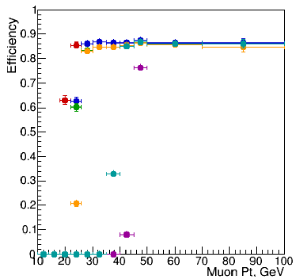
ENDCAP, Pt dependence
