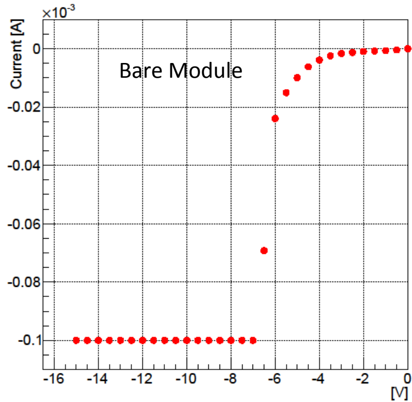
I-V Measure
