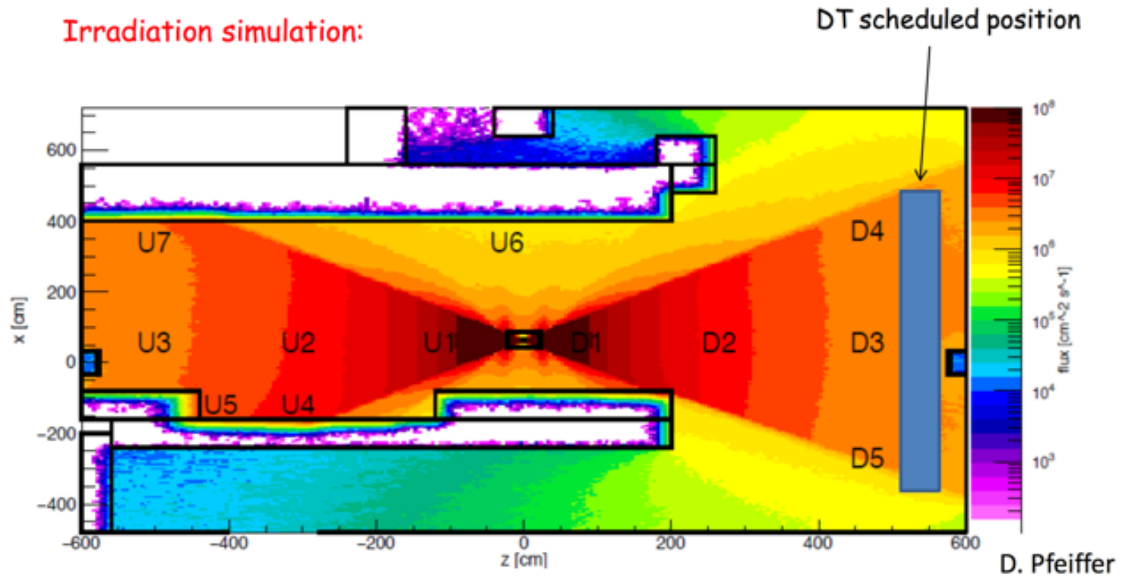
Total flux of gamma from ^{137}\text{Cs} source
