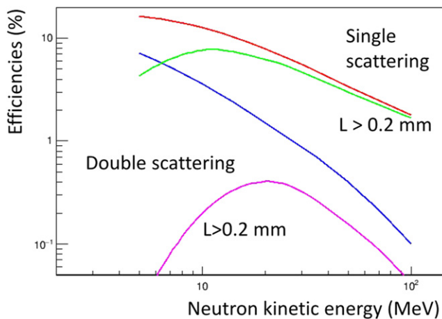
Figure 2. Probability of interaction and detection efficiency for neutrons as a function of the kinetic energy. The red line refers to single scattering into the cube; the green line refers to recoil proton ranges greater than 0.2 mm (minimum detectable). The blue line refers to double neutron scattering into the cube, while the purple line is obtained requiring that both recoil protons have a range greater than 0.2 mm.
