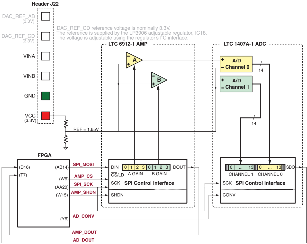
Figure 9-2: Detailed View of Analog Capture Circuit
