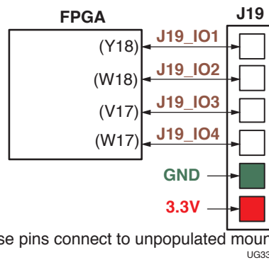
Figure 15-9: FPGA Connections to the J19 Accessory Header
