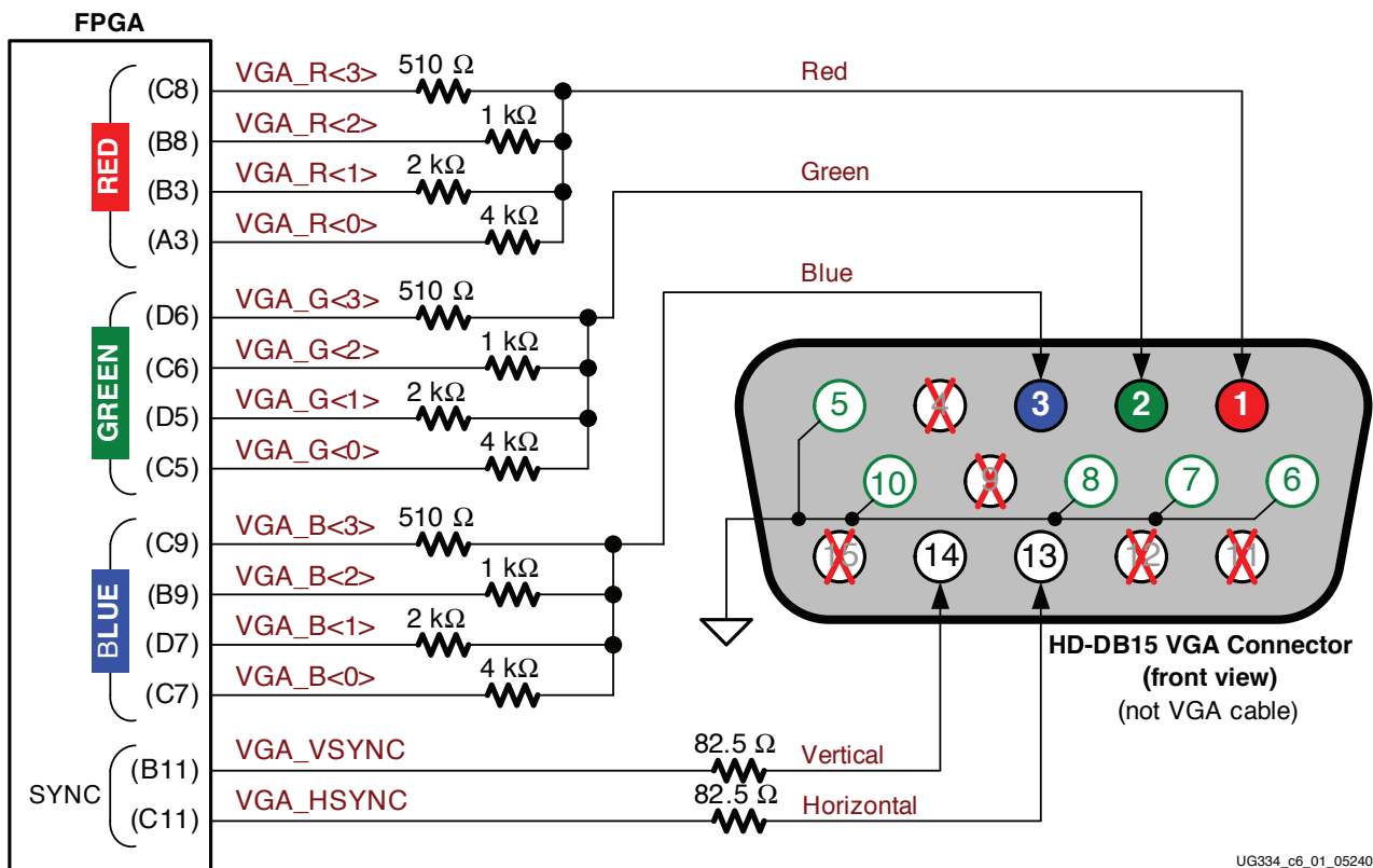
Figure 6-1: VGA Connections from the Starter Kit Board
