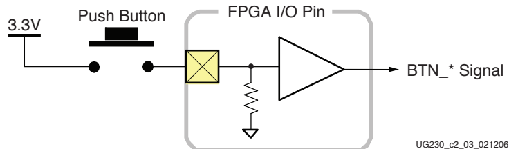
Figure 2-6: Push-Button Switches Require an Internal Pull-Down Resistor in the FPGA Input Pin
