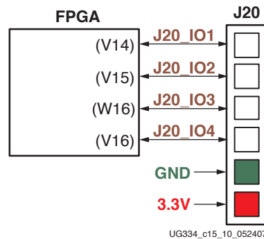
Figure 15-10: FPGA Connections to the J20 Accessory Header
