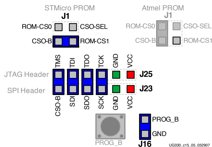
Figure 12-4: Jumper Settings for Direct SPI Flash Programming
