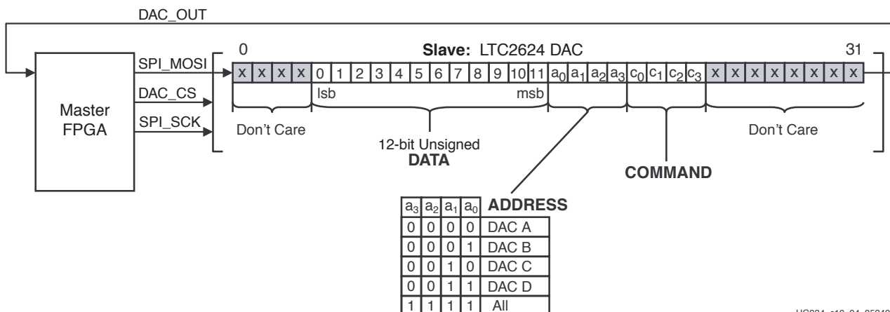
Figure 10-4: SPI Communications Protocol to LTC2624 DAC
