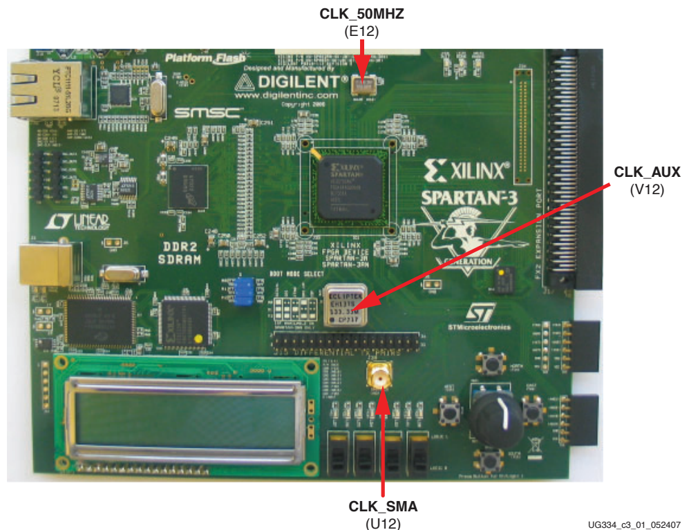
Figure 3-1: Clock Sources on Starter Kit Board
