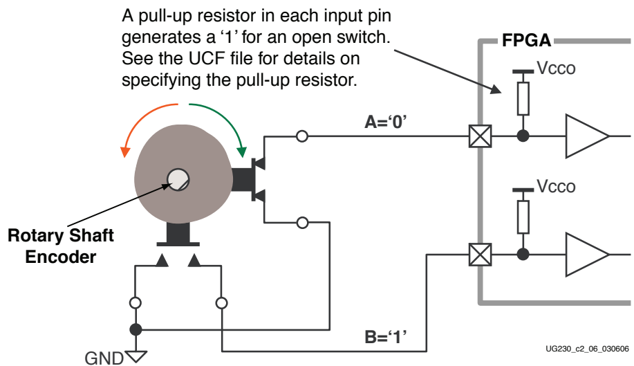
Figure 2-9: Basic Example of Rotary Shaft Encoder Circuitry
