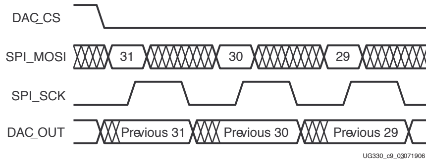
Figure 10-3: SPI Communication Waveforms
