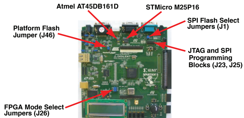
Figure 12-1: SPI Serial Flash PROMs and Associated Jumpers
