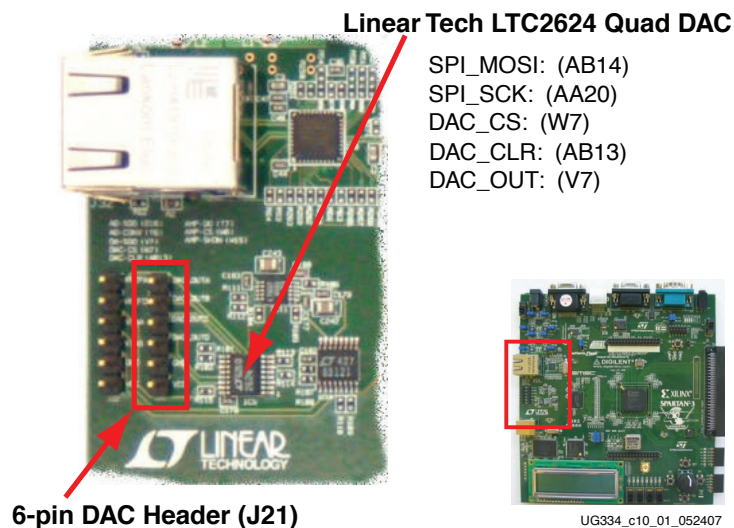
Figure 10-1: DAC and Associated Stake Pin Header (J21)
