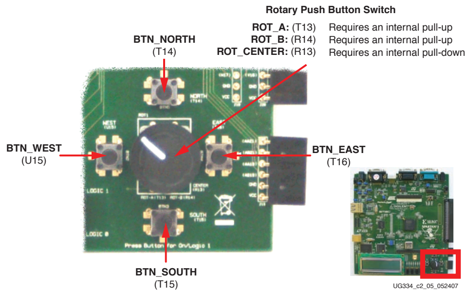
Figure 2-5: Four Push-Button Switches Surround the Rotary Push-Button Switch
