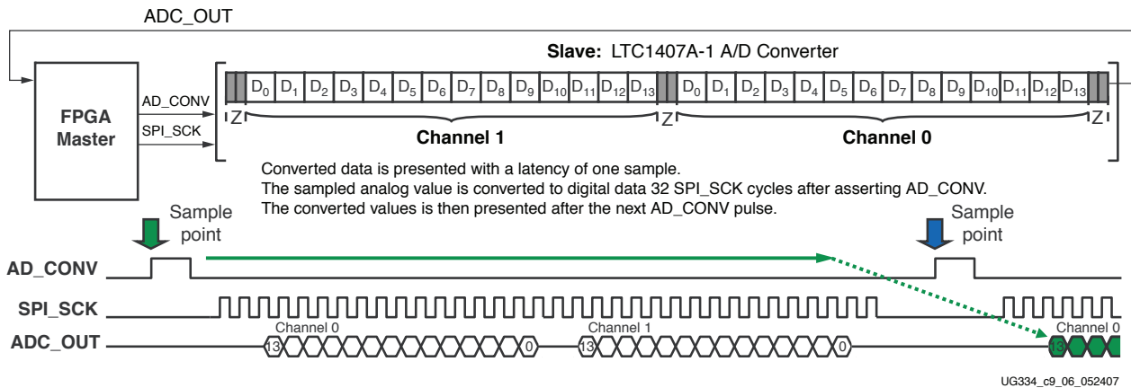
Figure 9-6: Analog-to-Digital Conversion Interface
