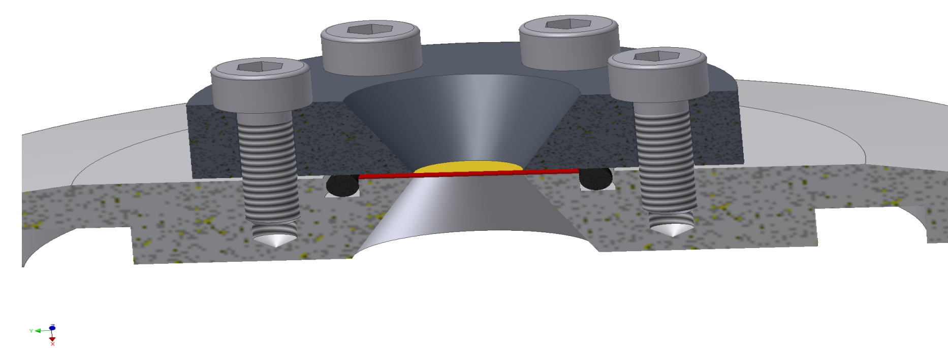
Cross-section schematic of exit flange ( \varnothing 4 \text{ cm} ): sealing O-ring (black), extraction foil (yellow) and optional mesh for support (red). Aperture size is 5 mm.
