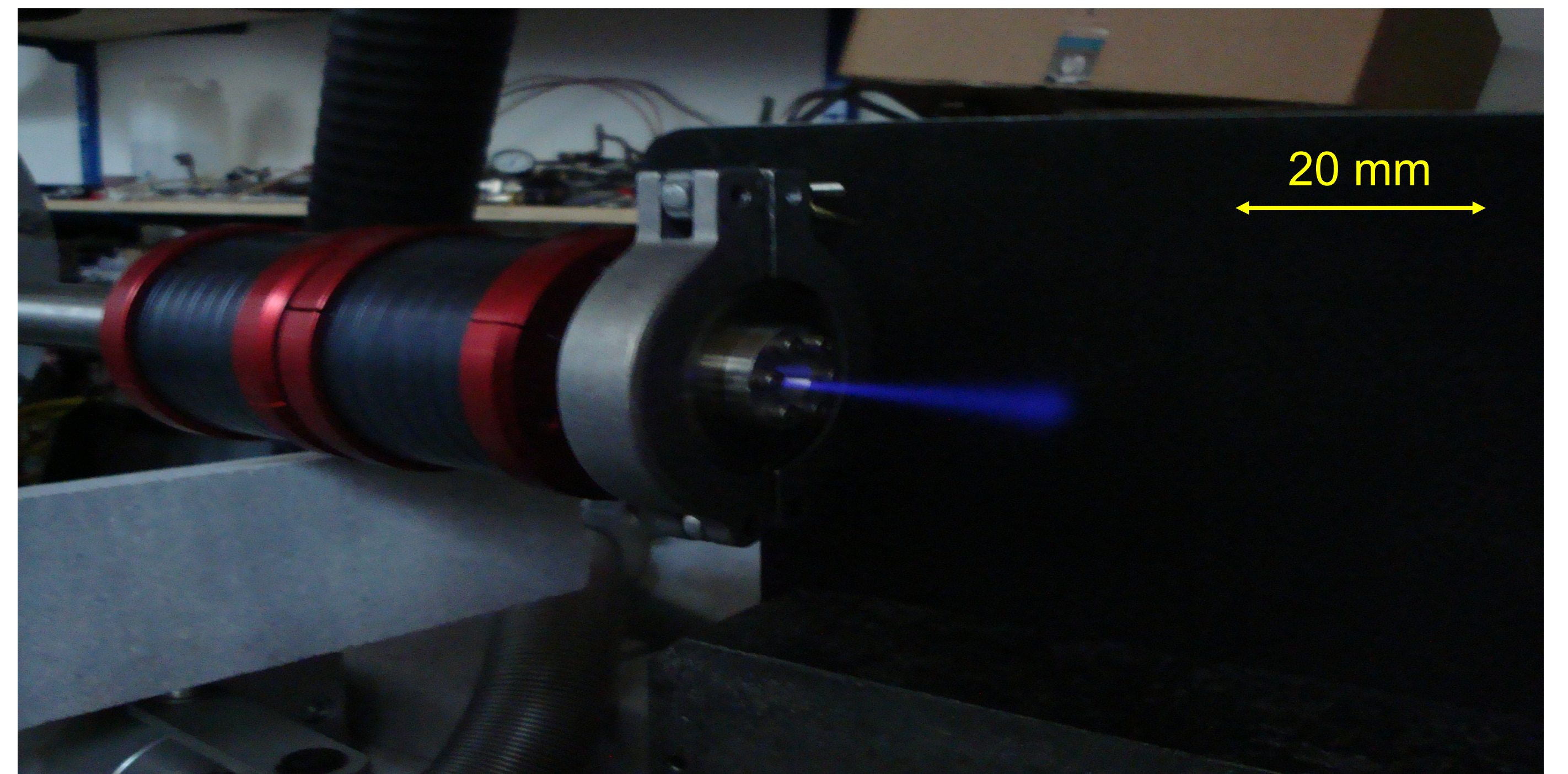
Beam extraction system: a vacuum-tight exit flange containing a 5 μm steel foil marks the end of the 2 MeV beam line. The H - ions pass through the foil, thereby being stripped of electrons and losing approx. 0.5 MeV kinetic energy. The extracted proton beam is visible by eye (blue glow) through excitation of the air. The beam continues depositing energy and starts to grow, the widest and brightest part at the end indicates the Bragg peak.
